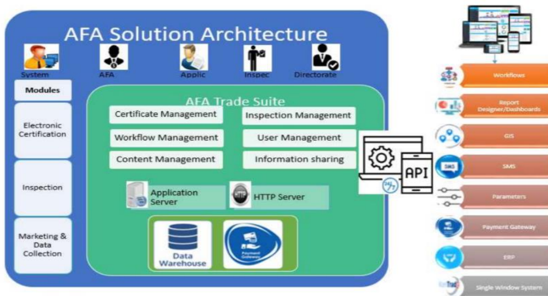
Figure 1 Solution Architecture
