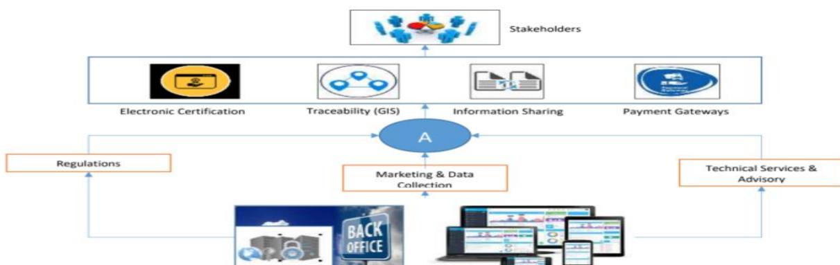
Figure 1 Solution Architecture
